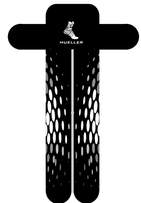
SHOULDER
